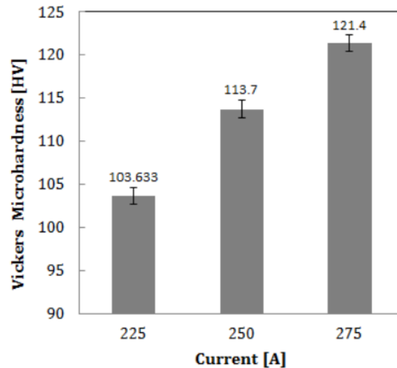
FIGURE 6. Vickers microhardness testing results.
