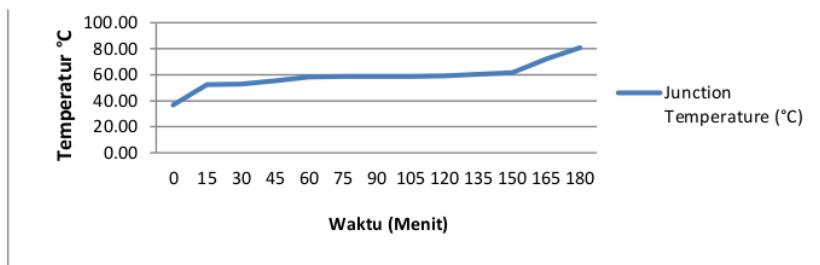
Gambar 5. Grafik junction temperature T_j NL500A.
