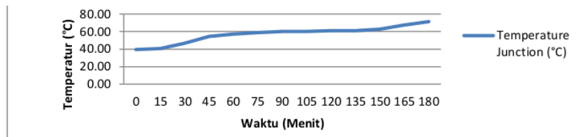
Gambar 9. Grafik junction temperature T_j NL500C.
