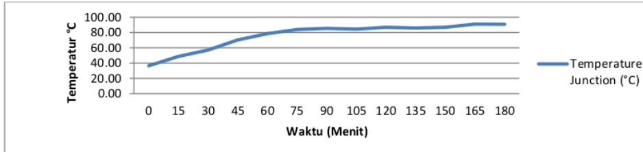
Gambar 7. Grafik junction temperature Tj NL500B
