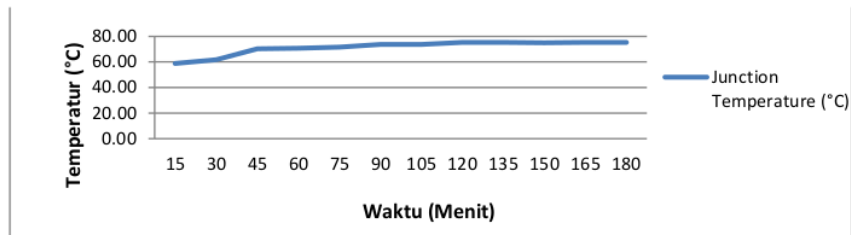
Gambar 11. Grafik junction temperature Tj NL500D.
