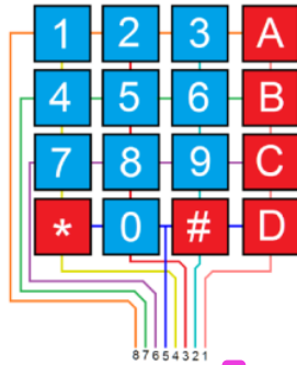
Figure 4. Keypad 4x4 Matrix Connections
