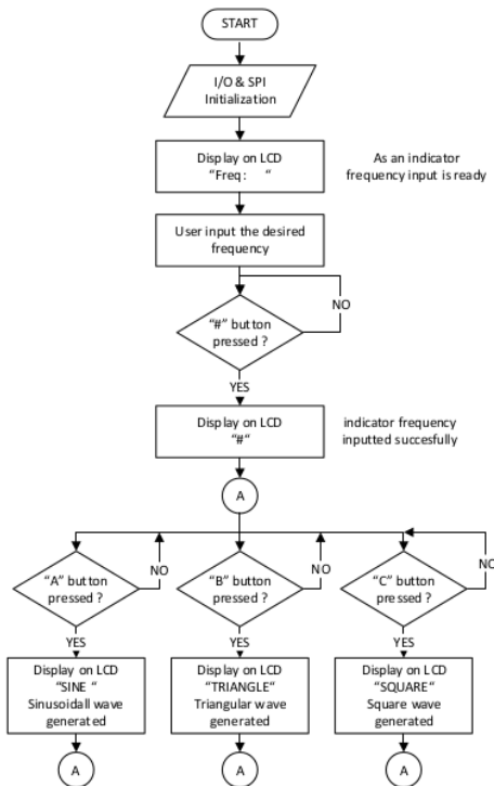
Figure 8. Program flow chart
