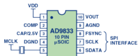
Figure 1. AD9833 Configuration
