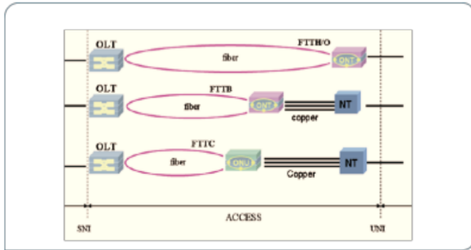
Fig. 5. FTTX applications model in PON technology [13].
